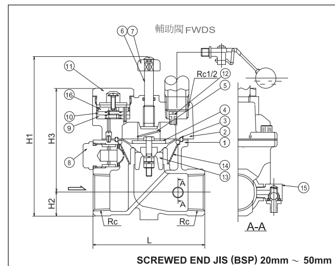
SREWED END JIS (BSP) 20mm ~ 50mm
